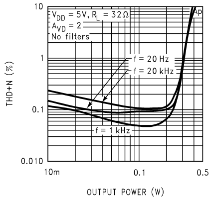
THD+N vs Output Power Bridged Power Amp
