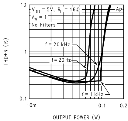
THD+N vs Output Power Line Out/HP Amplifiers
